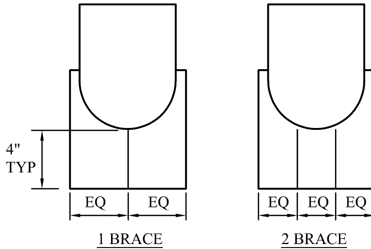
STRAIGHT ADAPTER BRACE DETAIL
