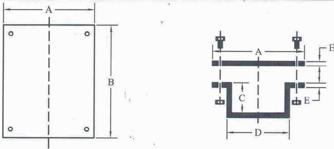
MECHANICAL COUPLING DETAIL
